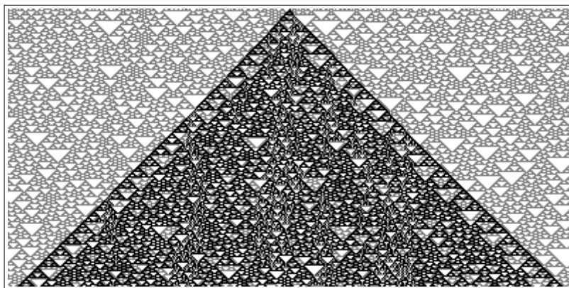
rule 126
